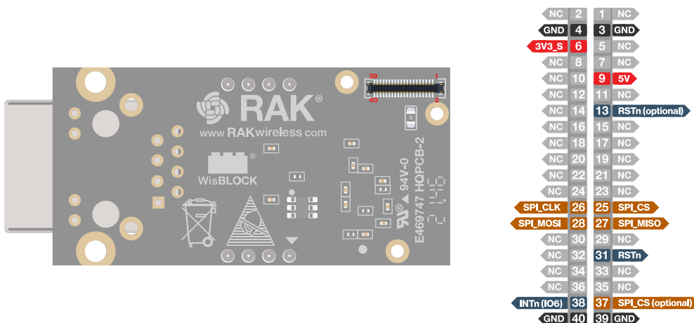
Figure 5: RAK13800 pinout
