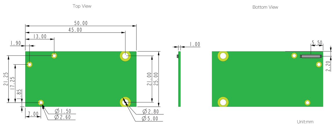
Figure 6: RAK13800 mechanical dimensions
