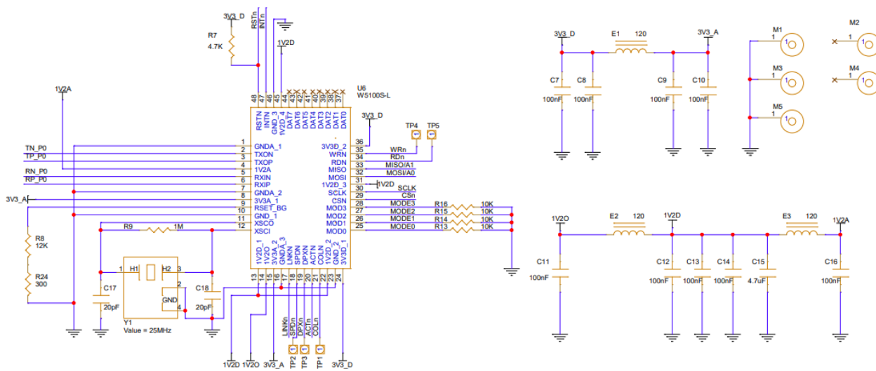
Figure 9: WIZnet W5100S-L Ethernet controller and mounting holes
